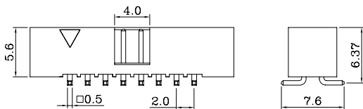
Vertical SMT/立贴
